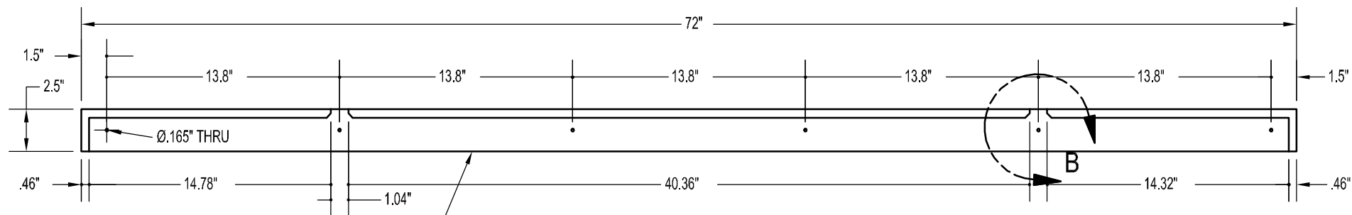
TOP TRIM BACK VIEW SCALE 1/8" = 1"
